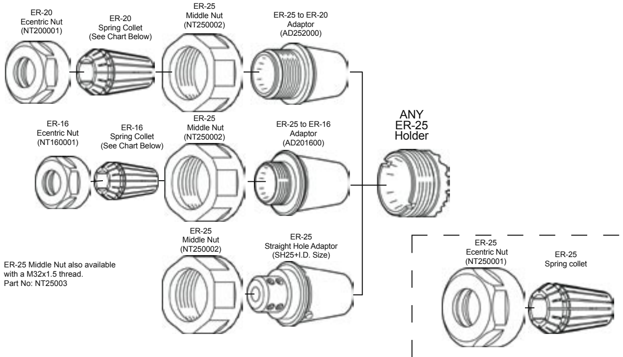
ER-16 Collets
