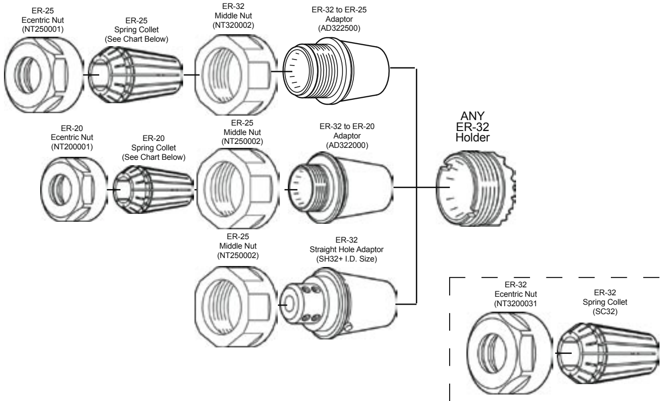
ER-20 Collets
